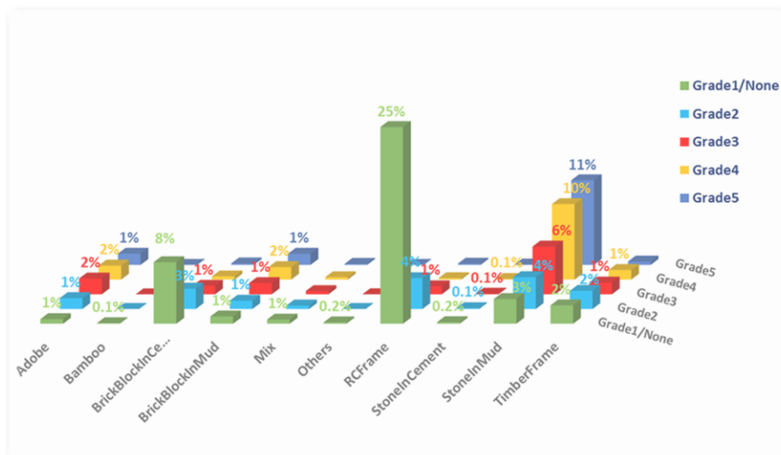
Figure 9: Overall Damage Grade Distribution vs Building Typology
