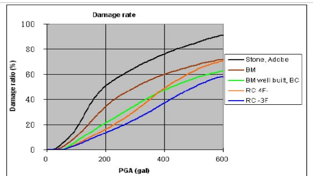
Figure 6: Building fragility functions modified by the project
