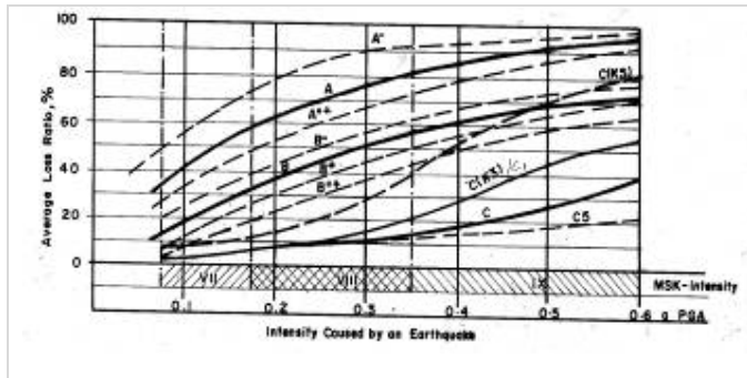
Figure 5: Building fragility functions given in Nepal National Building Code
