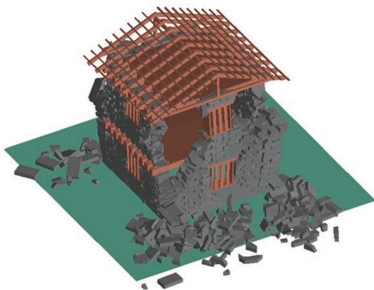
Unreinforced Masonry: AEM result @ 0.4 g
